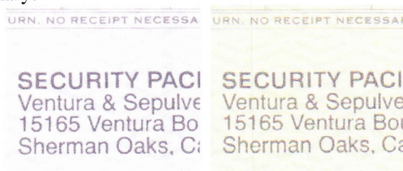
Figure 6. Grayscale.
