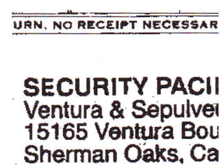
Figure 8. Binary image.
