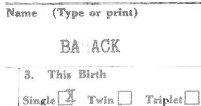
Figure 5. Obama's form
