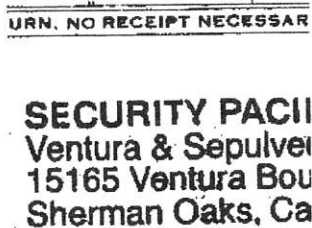
Figure 8. Binary image.
