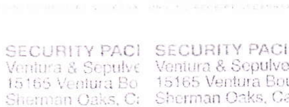
Figure 6. Grayscale.
